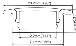
ABS-Profile 01
