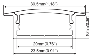
ABS-Profile 13
